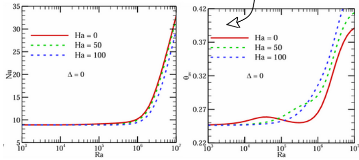
Quantitative Results
