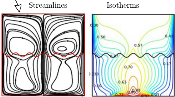
Qualitative Results
